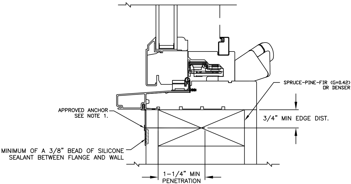
TYPICAL FLANGED WINDOW SILL
