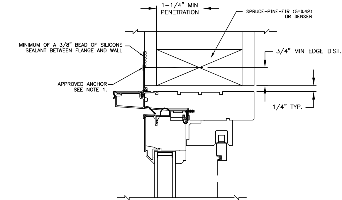
TYPICAL FLANGED WINDOW HEAD JAMB
